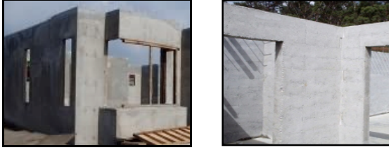
Figure 5: Foamed concrete as blocks and wall panels.
